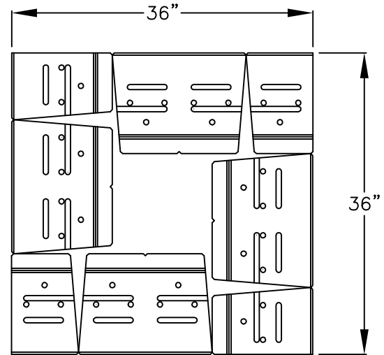
EVEN COURSE
