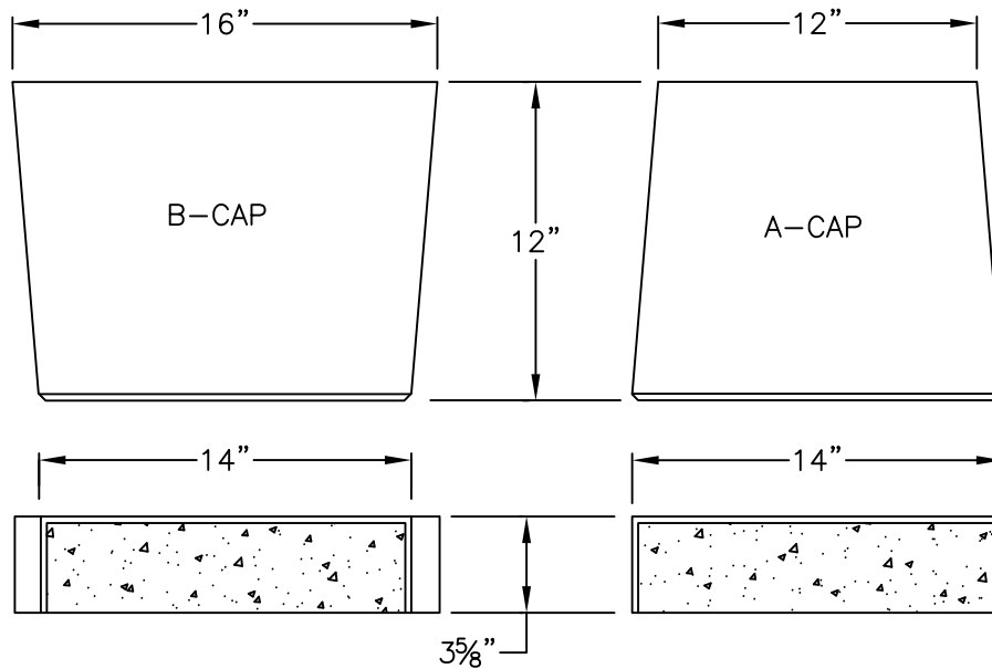
VERSA-LOK CAP UNITS UNIT DIMENSIONS SCALE: 1 1/2" = 1'
